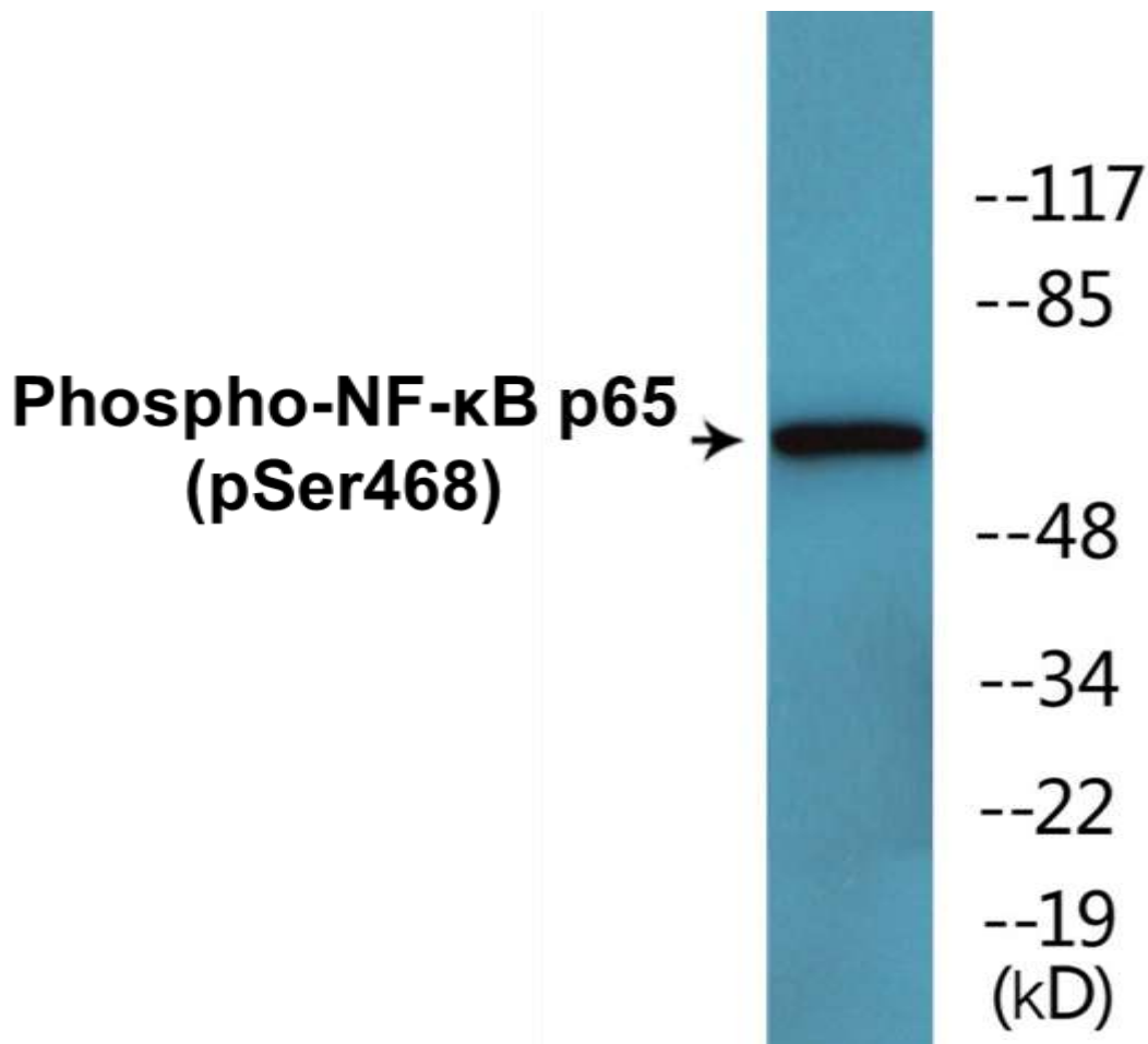
Figure 2. Western blot analysis of extracts from Jurkat cells and 293 cells, using the Anti-NF- \kappa B p65 (Phospho-Ser468) Antibody.
