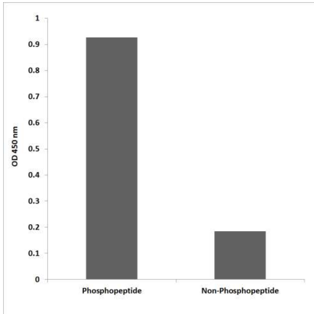
Figure 3. Enzyme-Linked Immunosorbent Assay (ELISA) for immunogen phosphor-peptide (left) and non-phospho peptide (right), using Anti-NF- \kappa B p65 (Phospho-Ser468) Antibody.
