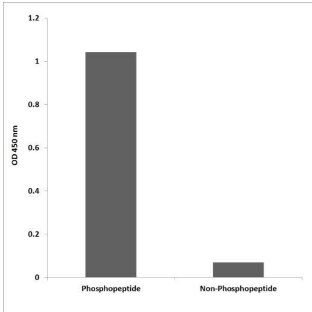
Figure 3. Enzyme-Linked Immunosorbent Assay (ELISA) for immunogen phosphor-peptide (left) and non-phospho peptide (right), using Anti-ETK (Phospho-Tyr40) Antibody.
